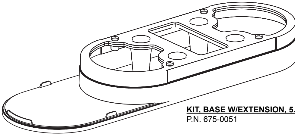
KIT, BASE W/OUT EXTENSION, 5.75" URN P.N. 675-0050
